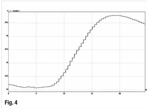
Fig. 4_Temperature increase at 3 W.
